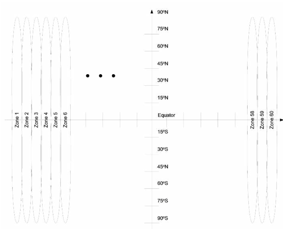
Figure B-1: Layout of UTM Zones
